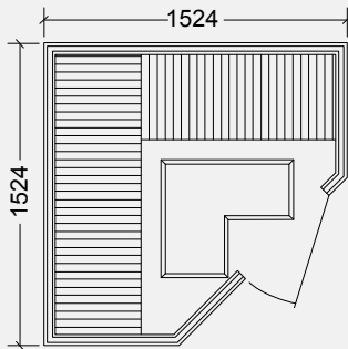
LUXUS 80-S LAYOUT
